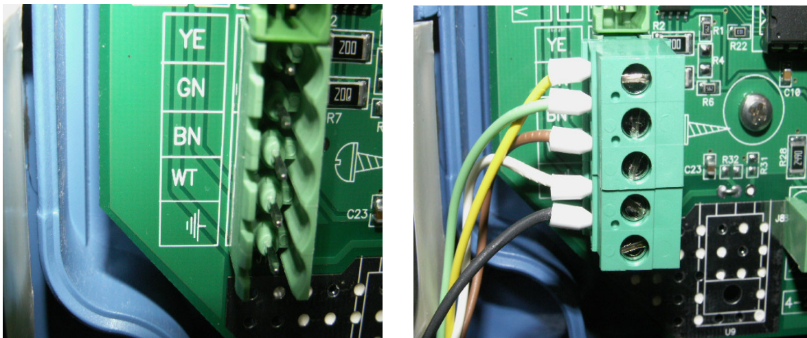
Figure 2: Connecting Turbidity Sensor to Turbidity Module
