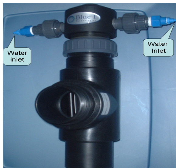
Figure – 2, bubble removal Mounting orientation
