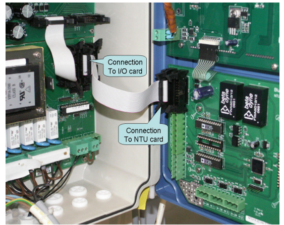
Figure 1: Connecting Turbidity Module to I/O Module
