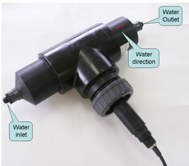
Figure – 1, standard flow cell Mounting orientation
